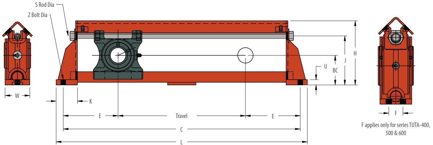
Figure 4.5 TUTA Drawings
