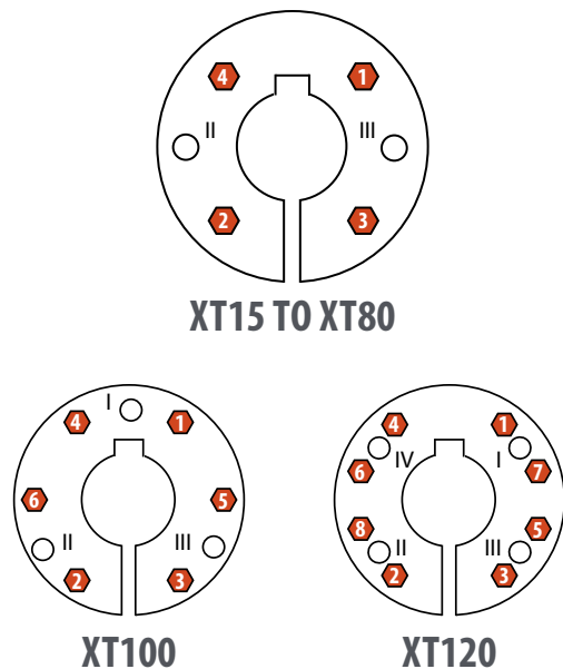
Figure 5.1 Numbered Capscrew Sequence
