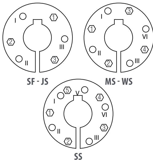
Figure 5.2 Numbered Capscrew Sequence
