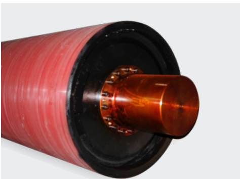
TURBINE END DISC / KEYLESS LOCKING DEVICE
