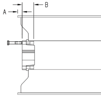
FIGURE 2.2 Bushing location wing pulleys
